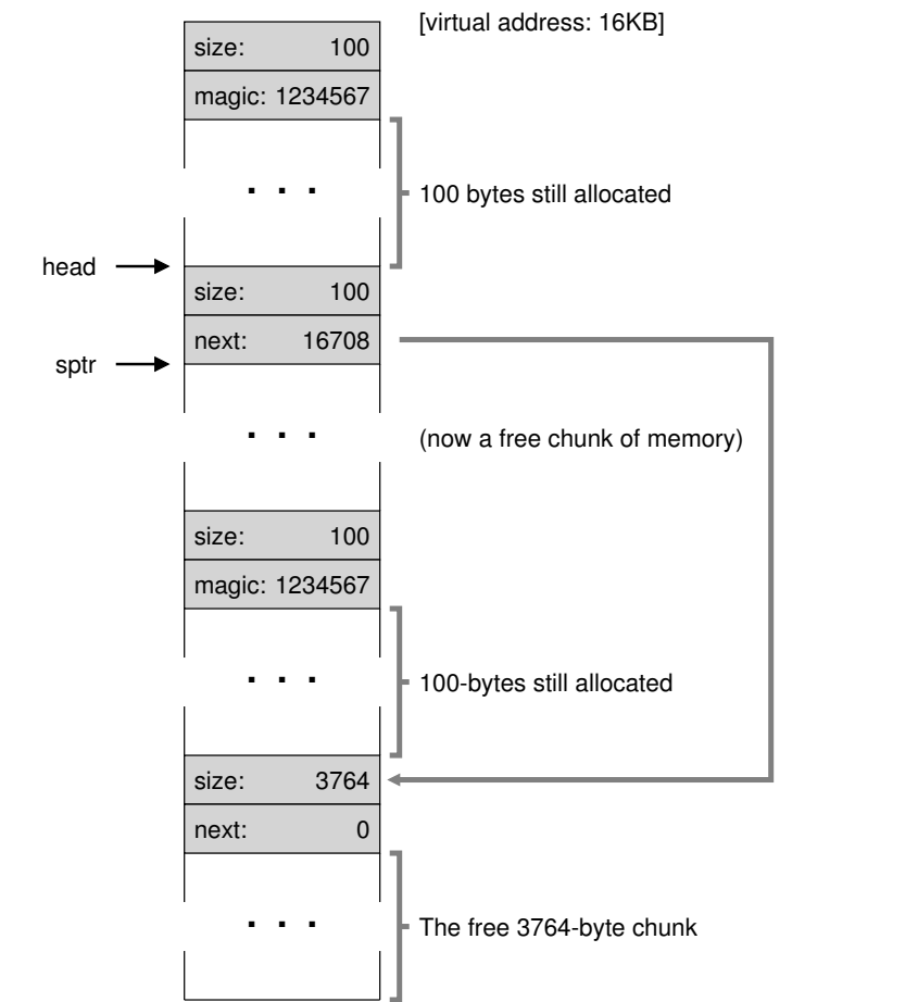
Figure 17.6: Free Space With Two Chunks Allocated
